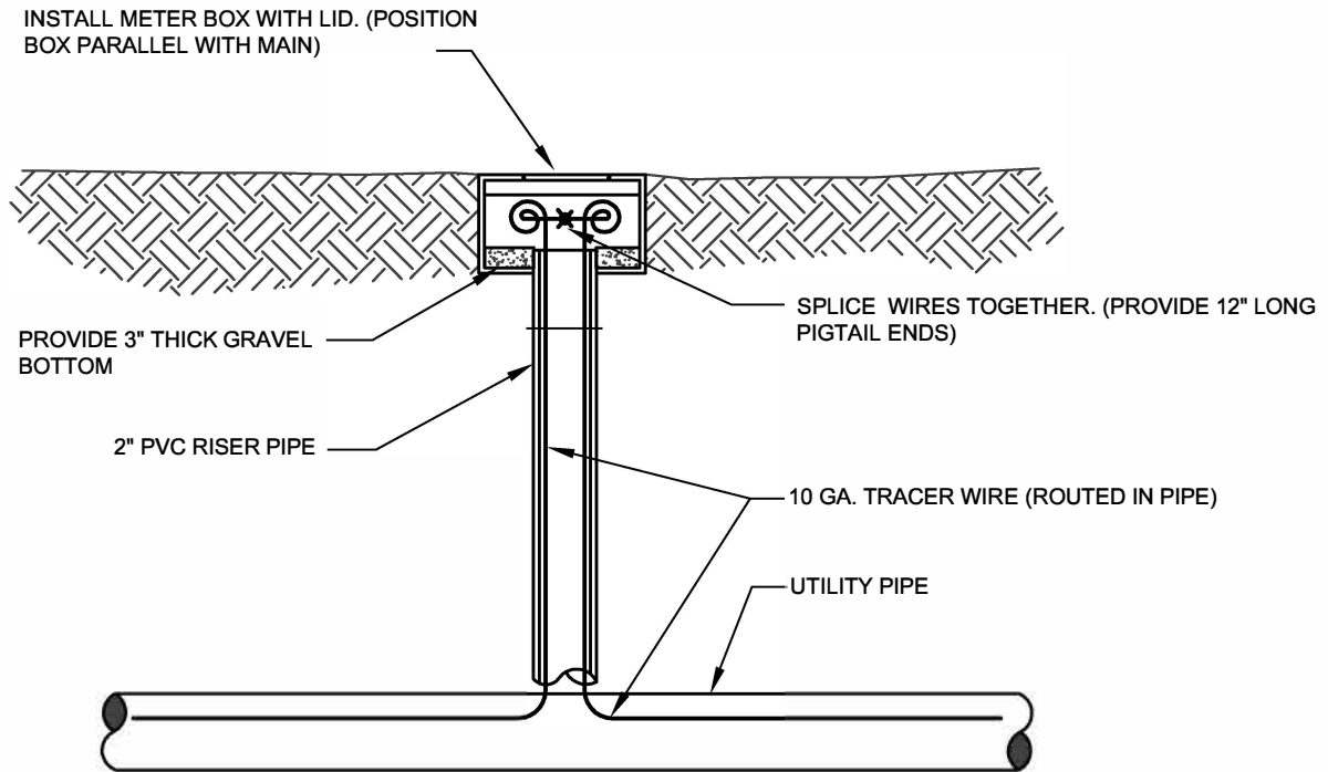
TRACER WIRE BOX UTILIZING METER BOX
