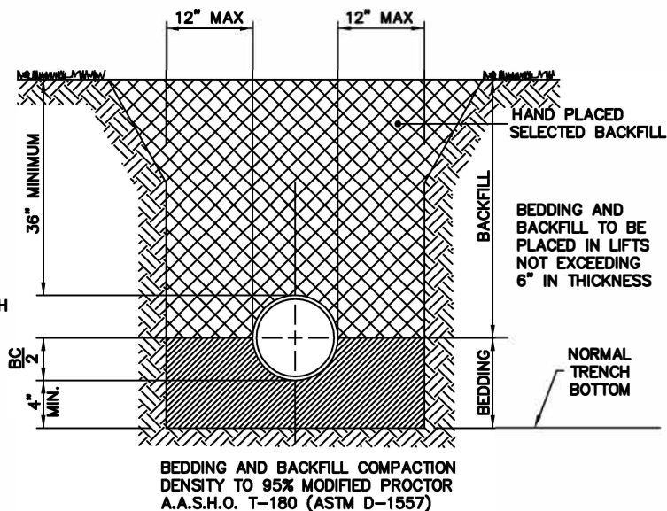
SANITARY SEWER PIPE BEDDING
