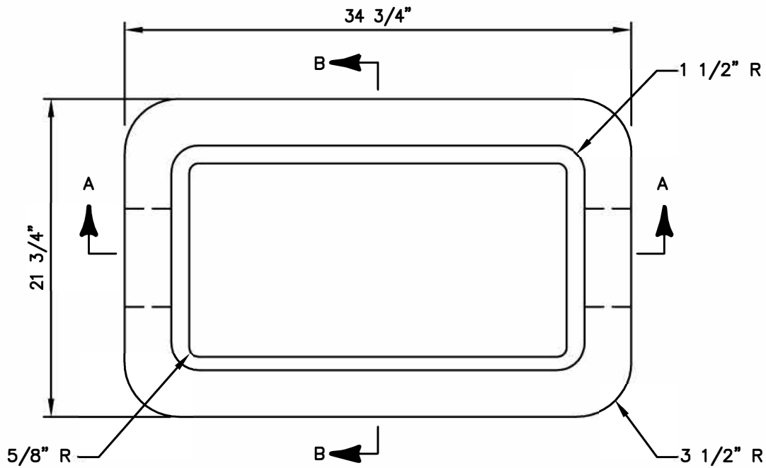
PLAN VIEW
