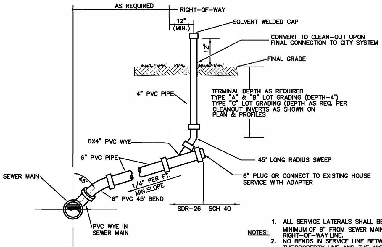
SIDE VIEW
