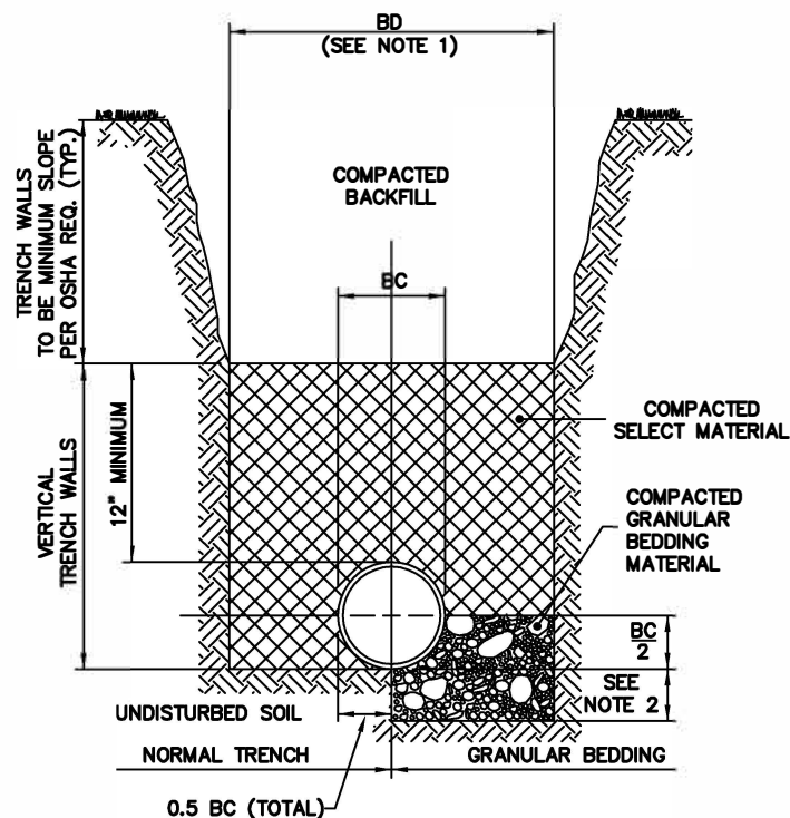
CLASS "B" BEDDING NORMAL CONDITIONS
