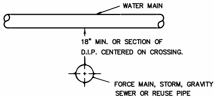
CROSSING SECTION
