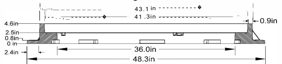
SECTION A-A FRAME VIEW
